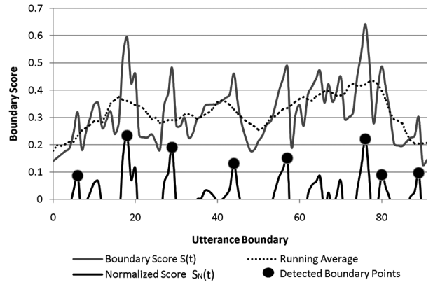
Figure 3: This figure summarizes how to locate boundaries with the scoring scheme. Initially the boundary score S(t) is calculated, whose value is subtracted by the running average to obtain the normalized score S_N(t) . We have the a priori knowledge that the number of story boundaries is eight, and therefore the eight highest local maxima are selected as the story boundaries.
