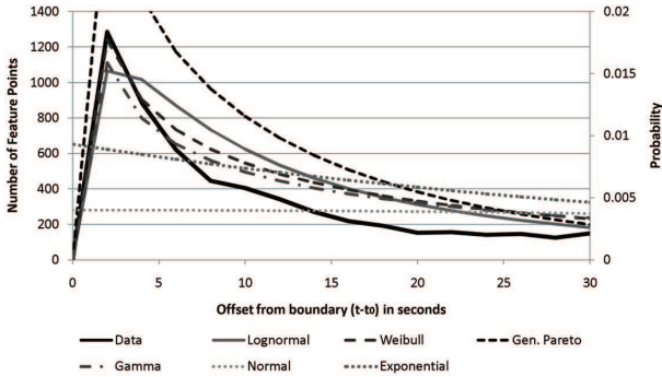
Figure 1: This graphs shows an example of the distribution of feature points (in this case, the feature points shown are the chain starts following real boundaries in long programs) and the hypothesized distributions (Normal, Exponential, Generalized Pareto, Gamma, Weibull and Log-normal). The hypothesized distributions are parameterized at their maximum likelihood estimation of the data. It is clear that normal and exponential distributions do not appear to fit the data well, while the other four distributions have shapes more similar to the distribution of real data. In this example, the best fit is by the Weibull distribution while the second best fit is by the log-normal distribution (data shown in Table 1).
