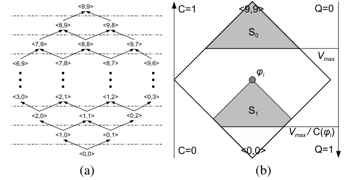
Fig. 1. Pruning on dependent attributes
